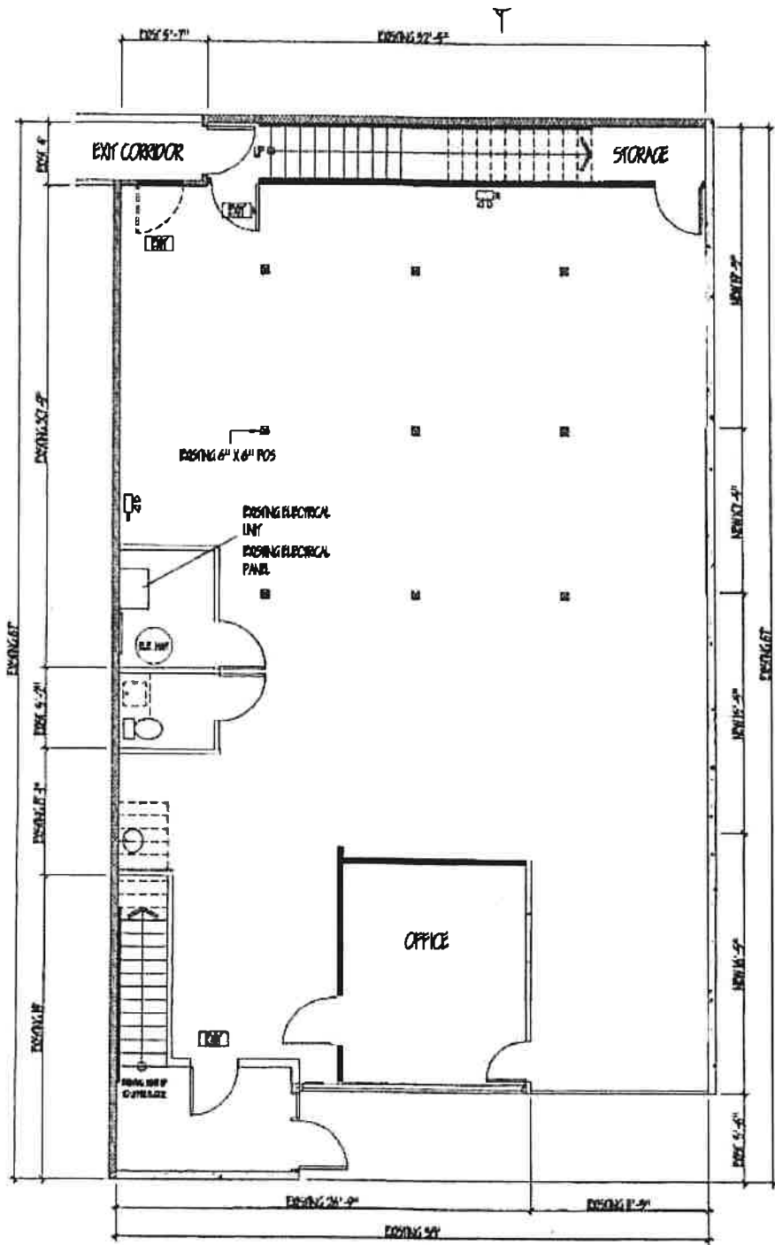
GROUND FLOOR PLAN V-10
