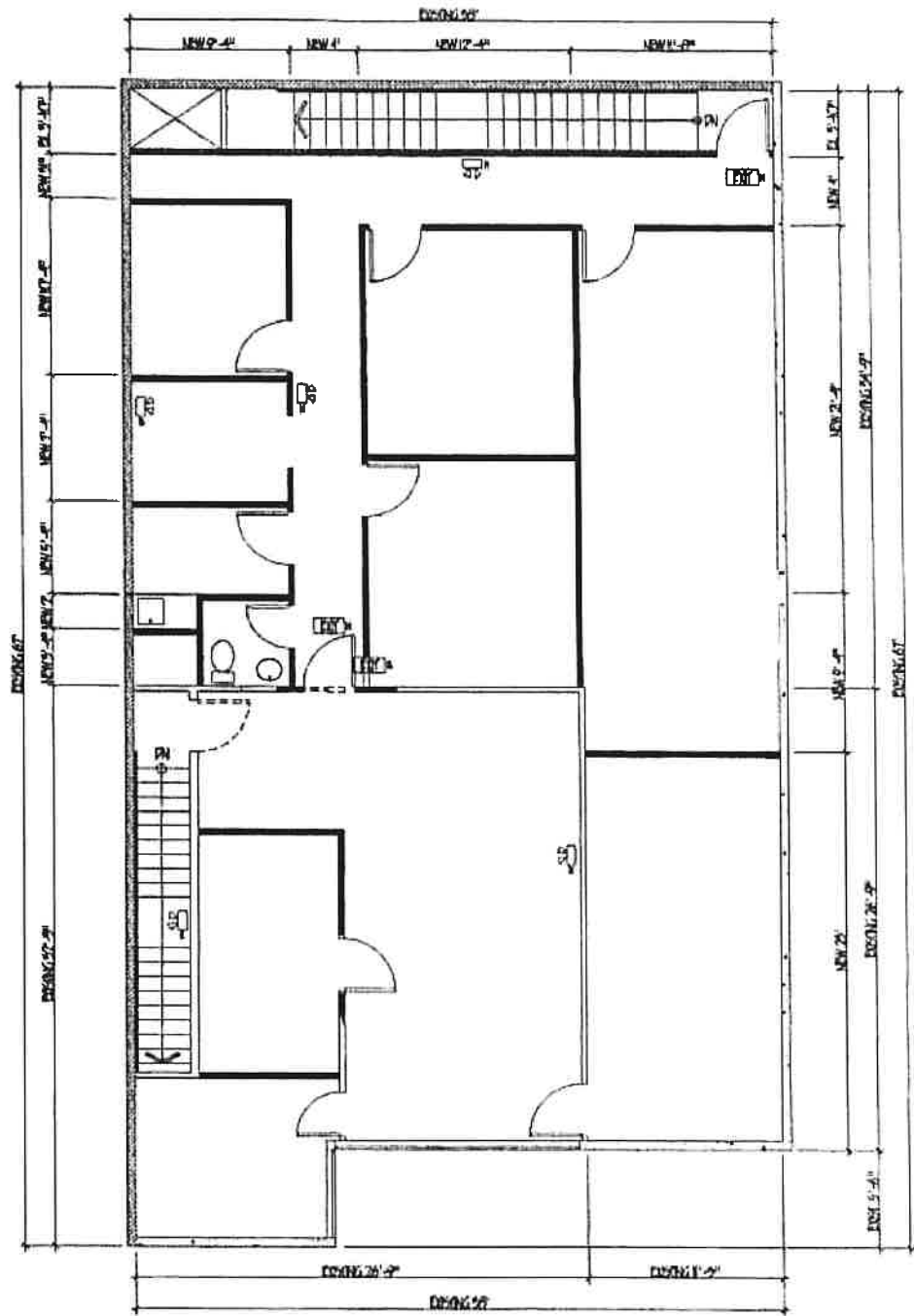
UPPER FLOOR PLAN V-10
