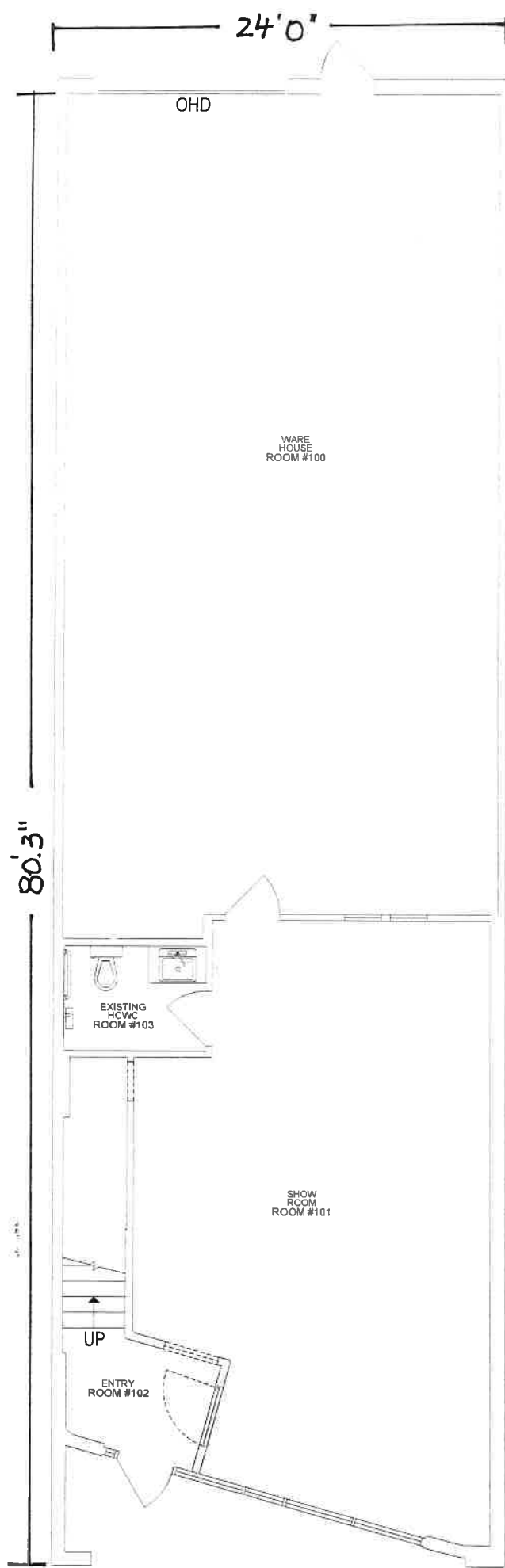
2 MAIN FLOOR PLAN SCALE: 1/4" = 1'-0"
