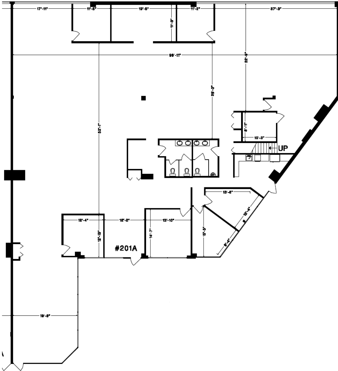
MAIN FLOOR
