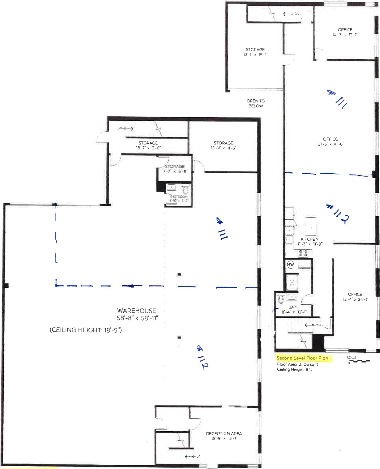
Ground Level Floor Plan Floor Area: 4,324 sq. ft. Ceiling Height: 8 ft.
