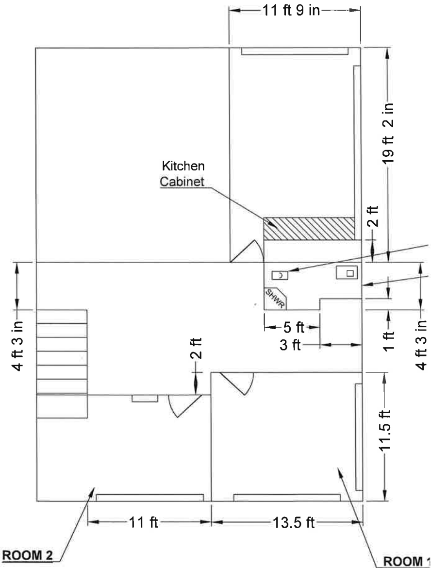
2nd Floor Layout Plan 1:100
