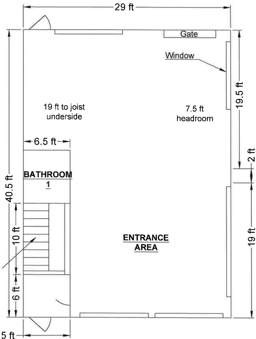
1st Floor Layout Plan 1:100
